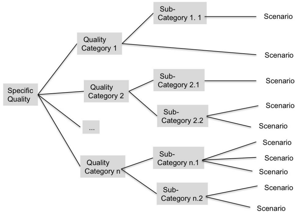
Figure 16: A generic schema for a quality tree
