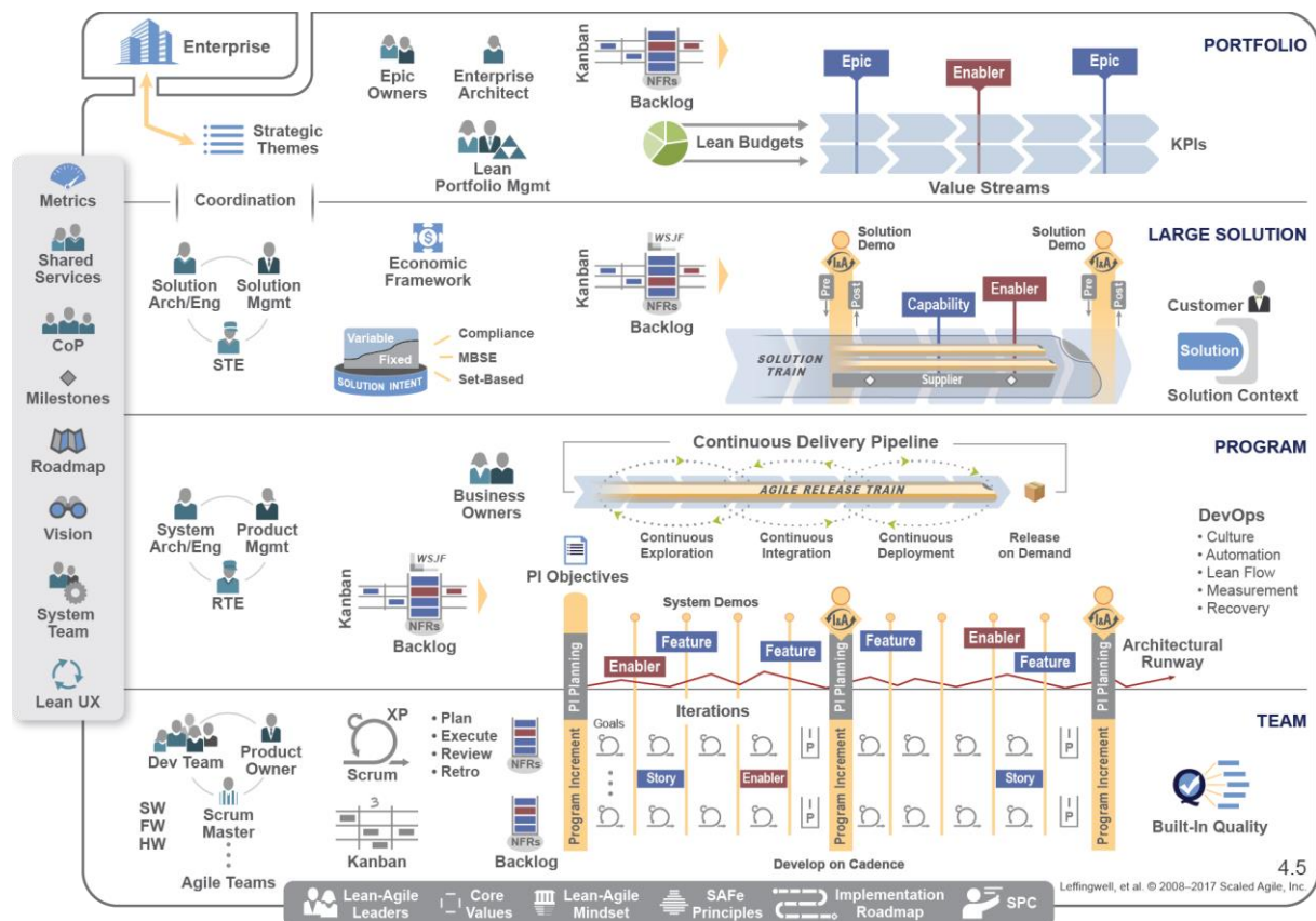
Figure 38: SAFe overview
