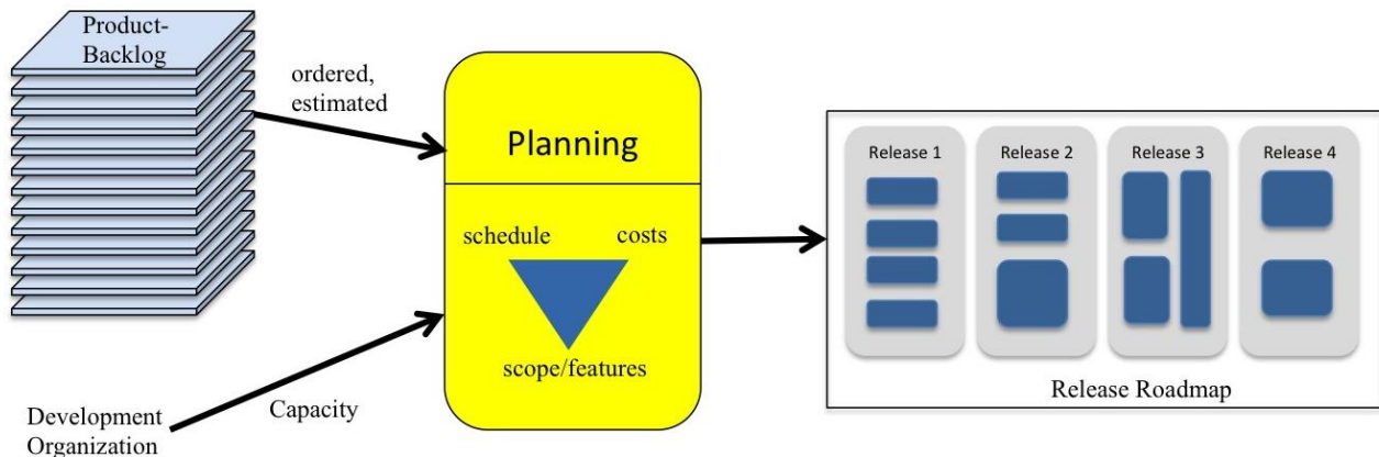
Figure 32: Release planning
