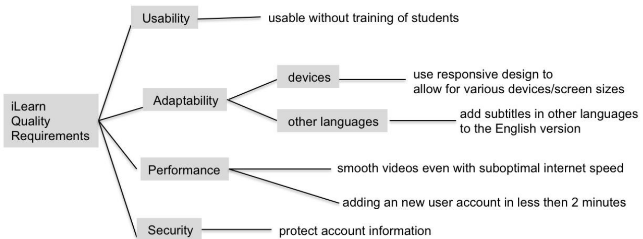
Figure 17: Parts of a quality tree for iLearn
